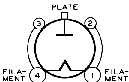
TUBE SYMBOL & TOP VIEW OF SOCKET CONNECTIONS
